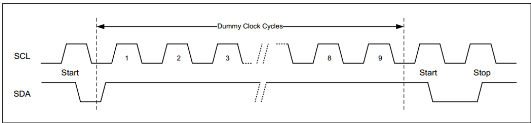
Figure 4 Soft Reset
