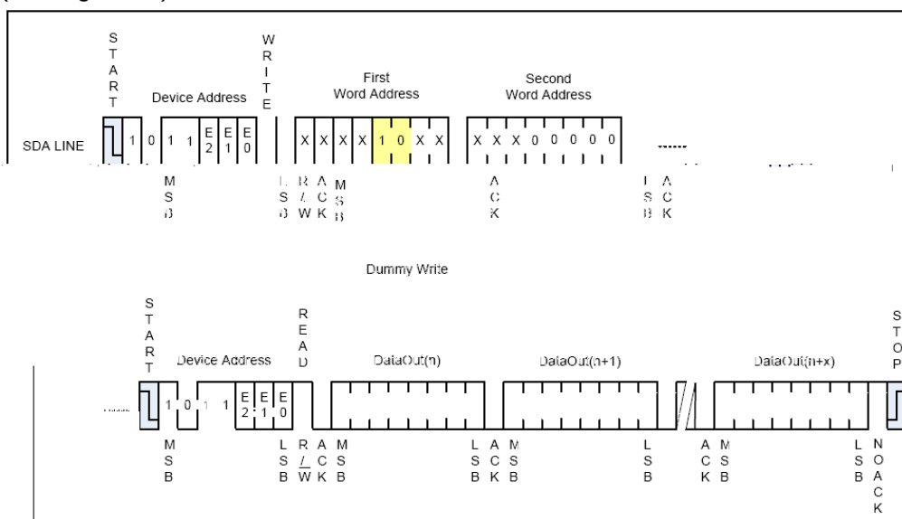
Figure 11 Sequential Read
