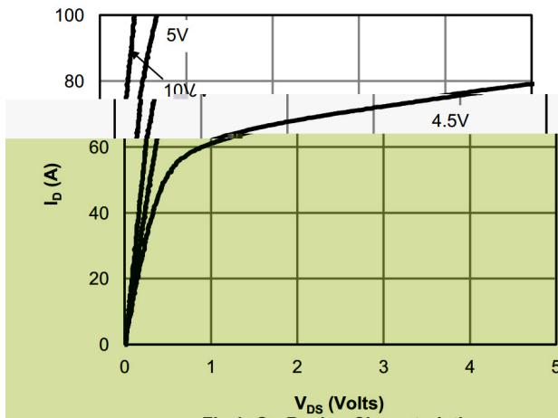
Figure 1: Drain Current Characteristics
