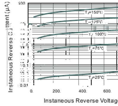
Fig.2 Typical Instantaneous Reverse
