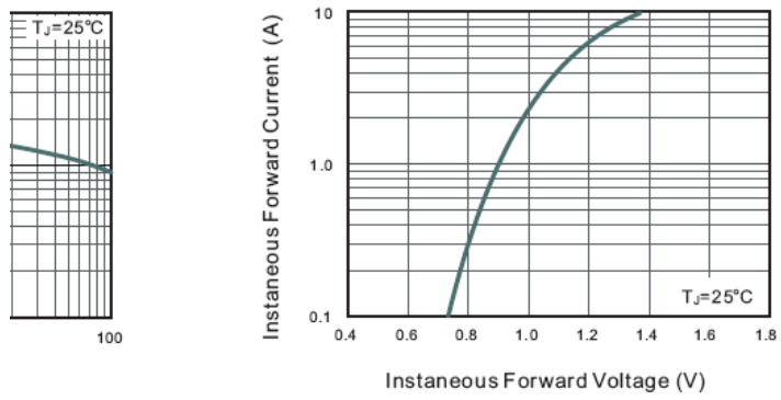
Fig.3 Typical Forward Characteristic
